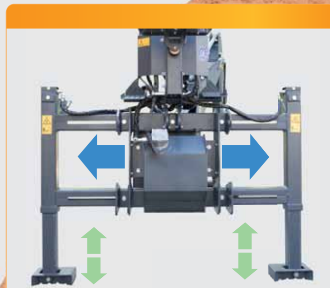
Independent stabilizer legs with remote-controlled locking valves. Our backhoes feature side-shift extension to optimize the equipment performance as well as the operator's safety in any working condition.
